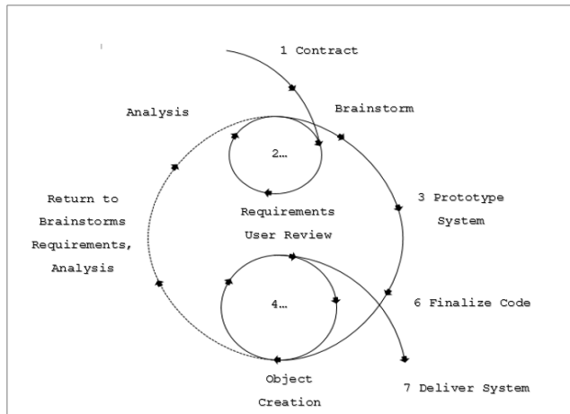
Figure 1. The Rapid Application Development Model
